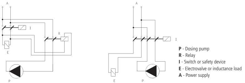
Fig. 11. Electrical installation.
